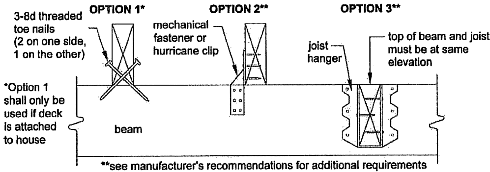
Figure 6: Joist-to-Beam Detail
