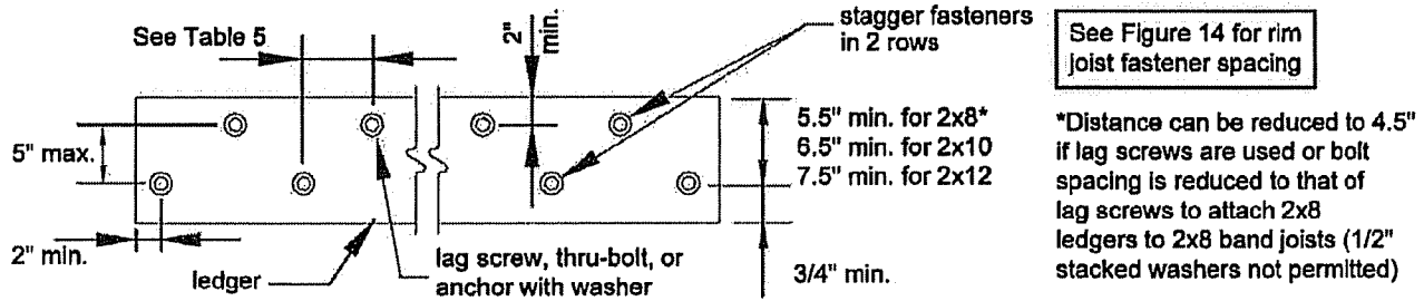
Figure 19: Ledger Board Fastener Spacing and Clearances
