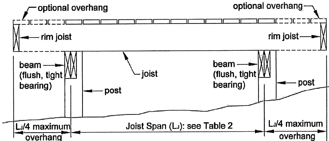
Figure 2. Joist Span – Free Standing Deck
