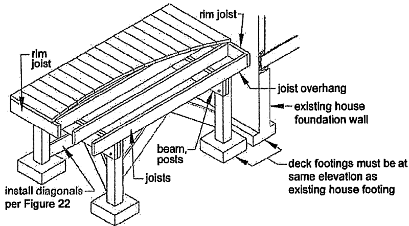
Figure 21. Free-Standing Deck
