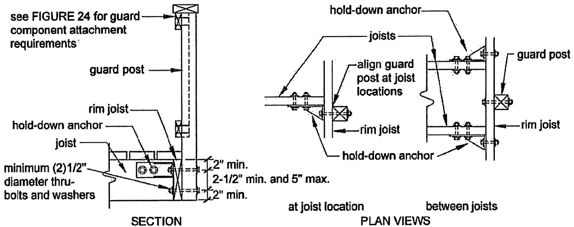
Figure 26. Guard Post to Rim Joist Example
