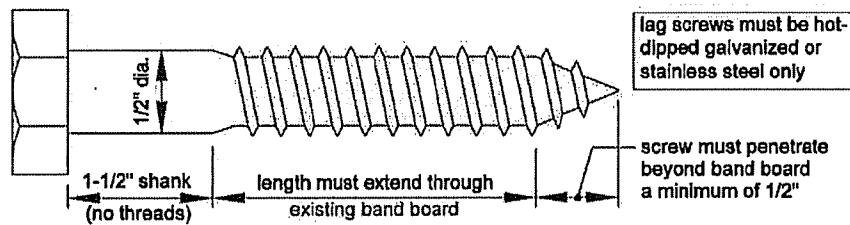
Figure 20: Lag Screw Requirements
